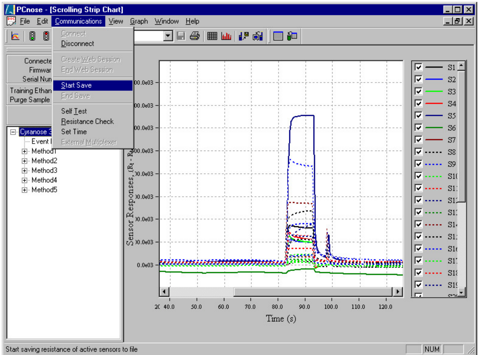
PCNose: Explorer Menu and Real-Time Sensor Array Response
